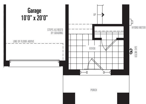
PARTIAL LOWER FLOOR PLAN ELEVATION B
