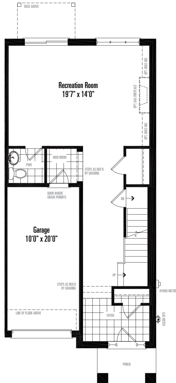
LOWER FLOOR PLAN ELEVATION A
