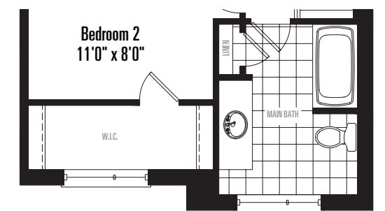
UPPER FLOOR PLAN ELEVATION A
