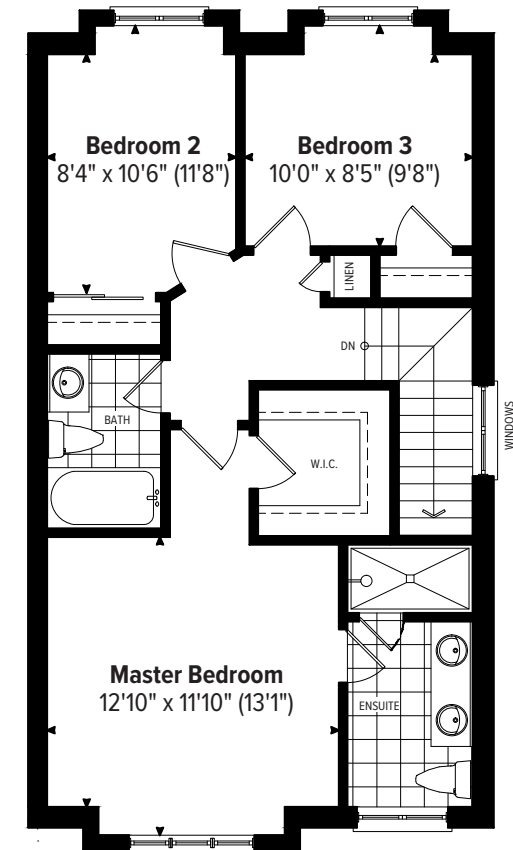
UPPER LEVEL FLOOR PLAN
