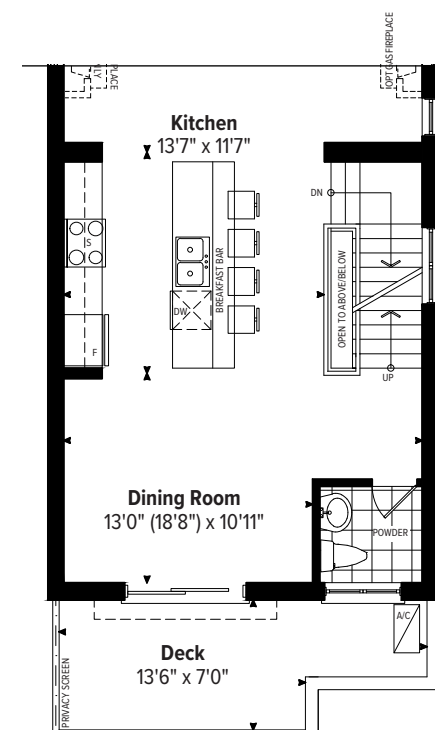
OPTIONAL MAIN LEVEL FLOOR PLAN
