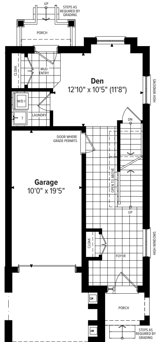
GROUND LEVEL FLOOR PLAN
