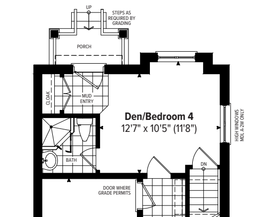
OPTIONAL GROUND LEVEL FLOOR PLAN
