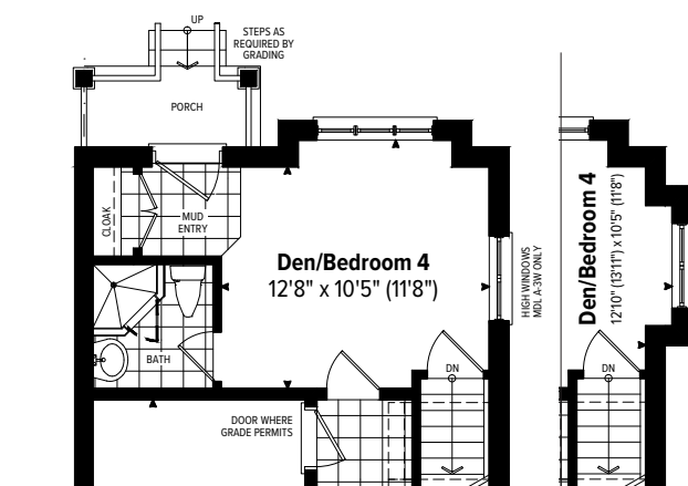
PARTIAL A3 END GROUND LEVEL FLOOR PLAN
