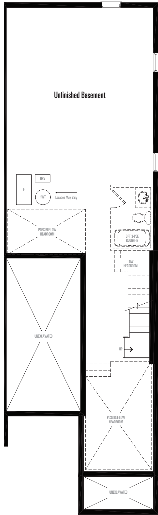
BASEMENT FLOOR PLAN ELEVATION A & B
