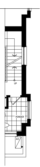
PARTIAL OPT. A3 END MAIN LEVEL FLOOR PLAN
