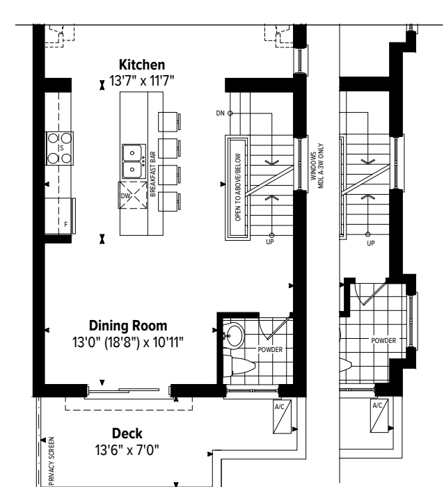
OPTIONAL MAIN LEVEL FLOOR PLAN
