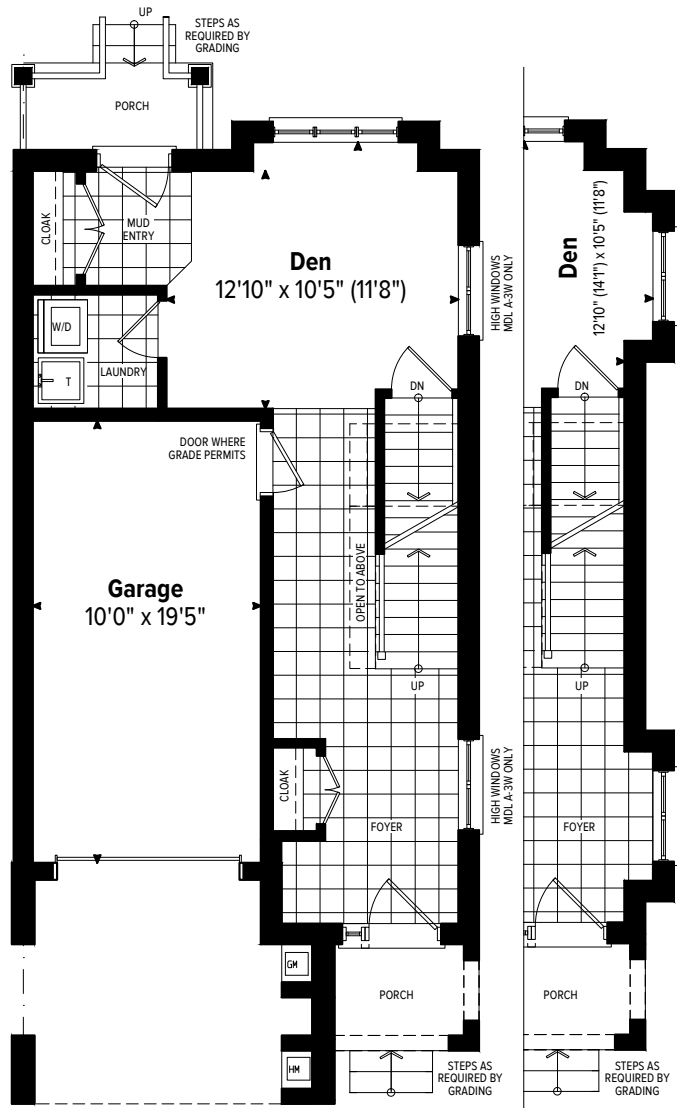
GROUND LEVEL FLOOR PLAN
