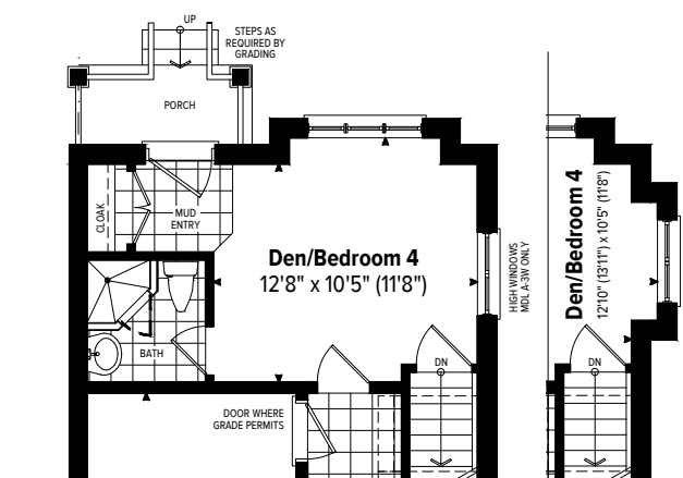
PARTIAL A3 END GROUND LEVEL FLOOR PLAN
